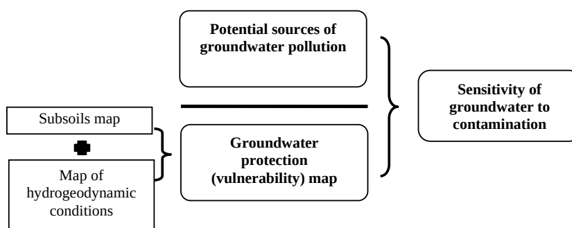
Figure 1. Conceptual framework for production a map of sensitivity groundwater to contamination
