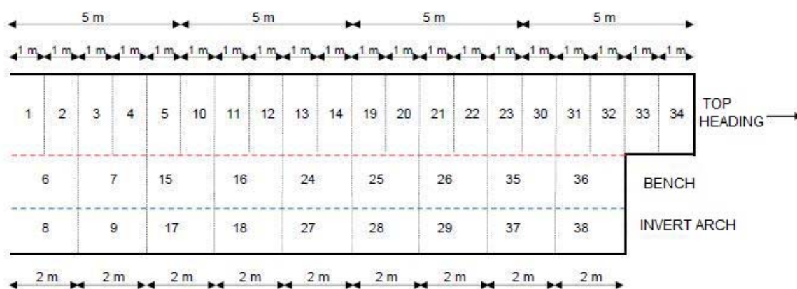
Figure 7. Three-stage profile excavation for 3D calculation
