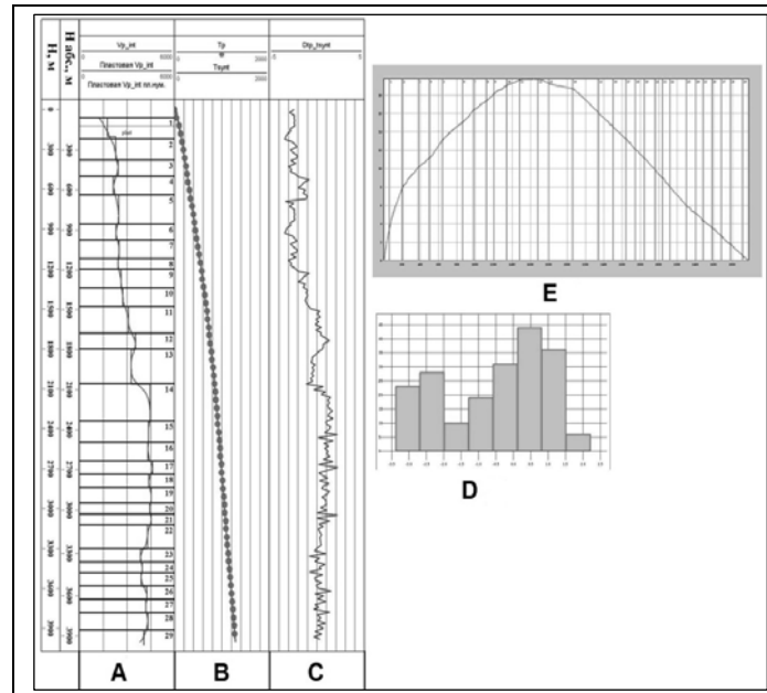
Figure 3. An example of layer velocity modeling.
